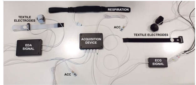
FIGURE 5. Acquisition device with the described hardware implemented in a compact way.
