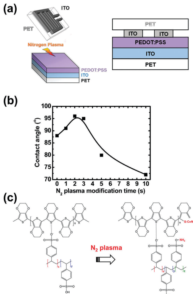
Fig. 4 (a) Schematic diagram of the PEDOT:PSS pressure sensor after N_2 plasma modification: different elements (left) and cross-sectional view of the final device (right). (b) Variation of the contact angle of PEDOT:PSS against the surface treatment time using N_2 plasma. (c) Molecular structure of PEDOT:PSS before and after surface modification using N_2 plasma. Reprinted and adapted with permission from J. Phys. Chem. C , 2016, 120 , 25977. Copyright 2016 American Chemical Society.
