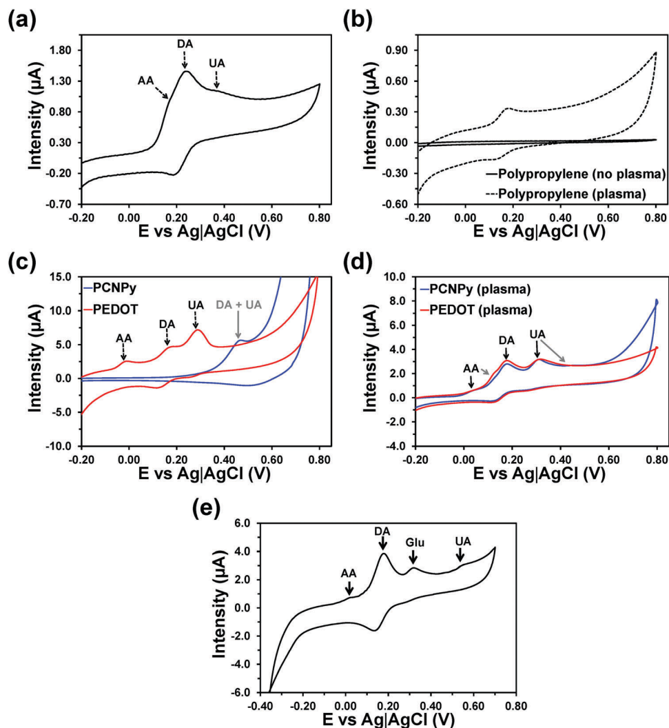
Fig. 11 (a) Control of 100 \mu\text{M} dopamine (DA), 100 \mu\text{M} uric acid (UA) and 100 \mu\text{M} ascorbic acid (AA) in 0.1 M phosphate buffer solution (PBS) at plasma-functionalized LPDE pressed onto a bare untreated glass carbon electrode (GCE). (b) Control voltammogram of 10 \mu\text{M} DA in 0.1 M PBS at plasma-functionalized polypropylene pressed onto a bare GCE. Voltammograms recorded using untreated electrodes (dashed lines) and cold-plasma treated electrodes (solid line) are displayed. The same behaviour was observed for plasma-functionalized polyvinylpyrrolidone, polycaprolactone and polystyrene. (c) Control voltammograms of DA, UA and AA (100 \mu\text{M} each) in 0.1 M PBS at untreated PCNPY- and PEDOT-modified GCEs. (d) Control voltammograms of DA, UA and AA (100 \mu\text{M} each) in 0.1 M PBS at plasma-functionalized PCNPY- and PEDOT-modified GCEs. Grey arrows in (d) indicate secondary oxidation processes. (e) Control voltammogram of 10 mM glucose (Glu) in 0.1 M PBS with 0.1 mM DA, 0.1 mM AA and 0.1 mM UA at plasma-functionalized LPDE pressed onto a GCE. In all cases, scan rate: 100 \text{mV s}^{-1} ; initial and final potentials: -0.40 V; reversal potential: +0.80 V.
