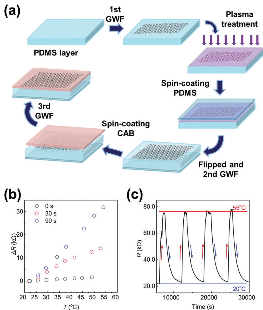
Fig. 5 (a) Schematic diagram of the assembly steps of the flexible temperature and humidity sensor. (b) Evaluation of the temperature sensing performance with different plasma treatment times. (c) Cyclic temperature tests. Adapted and reprinted with permission from ACS Appl. Mater. Interfaces , 2017, 9 , 30171. Copyright 2017 American Chemical Society.
