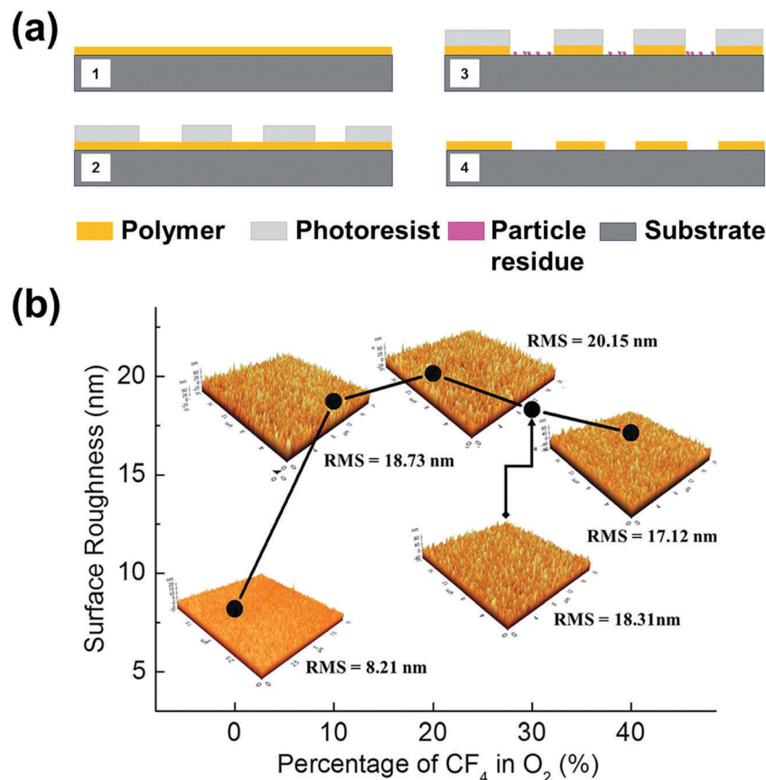
Fig. 6 (a) Schematic diagram showing the fabrication process of polymer etching by inductively coupled \text{CF}_4/\text{O}_2 plasma: (1) polymer deposition; (2) photoresist patterning; (3) polymer etching; and (4) residue removal and photoresist stripping. (b) Surface roughness of the polymer film measured using AFM relative to the different percentages of \text{CF}_4 in \text{O}_2 used for the inductively coupled plasma treatment. Reproduced from ref. 67 with permission from The Royal Society of Chemistry.
