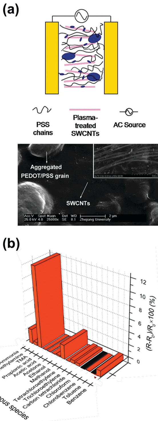
Fig. 9 (a) Scheme and SEM micrograph showing the structuration of PEDOT/PSS-SWCNTs composited by dielectrophoretic assembly. The SEM image of the structure was taken from ref. 87. SEM image reproduced from ref. 87 with permission from The Royal Society of Chemistry. (b) Selective responses of the dielectrophoretically assembled composite films with PEDOT/PSS and SWCNTs to various vapours of 10 ppm. Graphics reproduced from ref. 86 with permission from Elsevier B.V.
