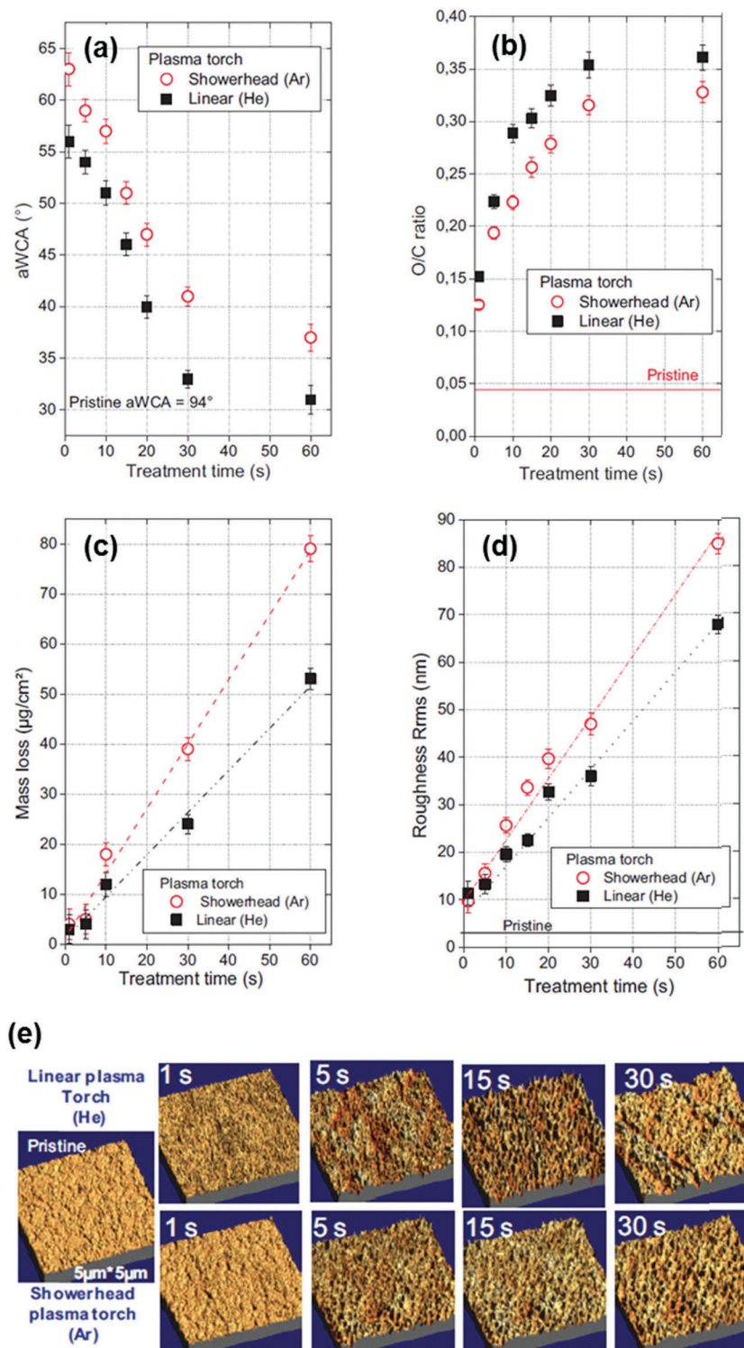
Fig. 3 Example of the influence of plasma treatments on the physical and chemical properties of polyethylene. Two different atmospheric plasma torches with different configurations (linear and showerhead supplied with He and Ar, respectively, as carrier gas) and different treatment times have been considered. The variation of the (a) advanced water contact angle (aWCA), (b) O/C ratio, (c) mass loss, (d) root-mean-squared roughness, and (e) surface topography as observed by AFM exposed to plasma torches with different configurations and treatment time is displayed. Reproduced from ref. 35 with permission from John Wiley and Sons.
