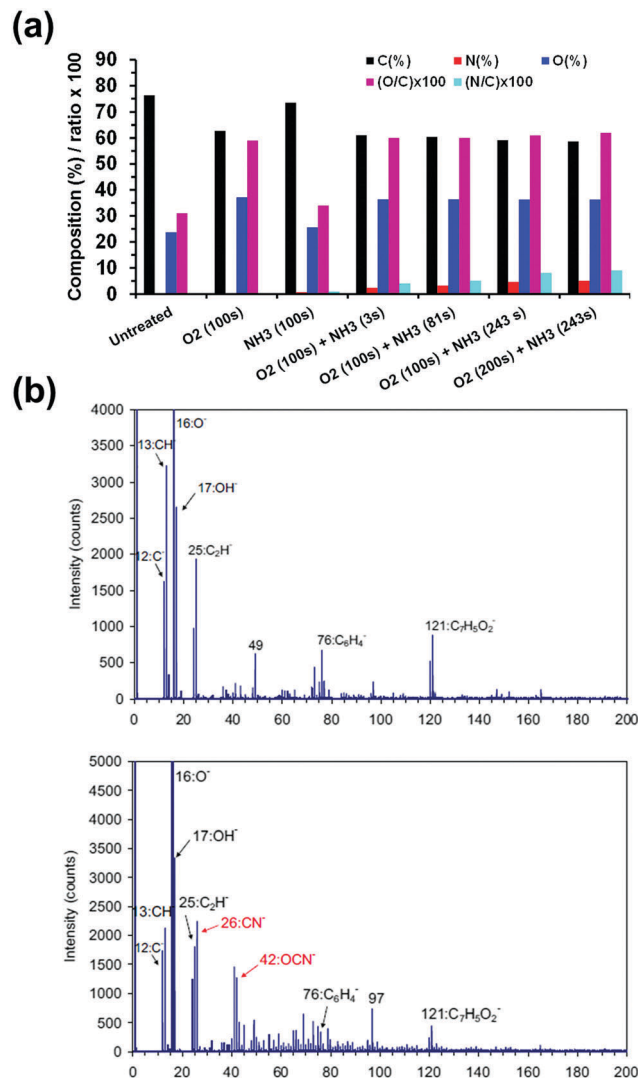
Fig. 7 (a) Variation of the composition (in atomic %) and atomic ratios ( \times 100 ) of untreated and plasma-treated PET fabrics as determined by XPS (presented data taken from ref. 81). (b) Negative time-of-flight secondary ion mass spectroscopy spectra of untreated (top) and O 2 and NH 3 plasma-treated (bottom) PET fabrics. Reproduced from ref. 81 with permission from Elsevier B.V.
