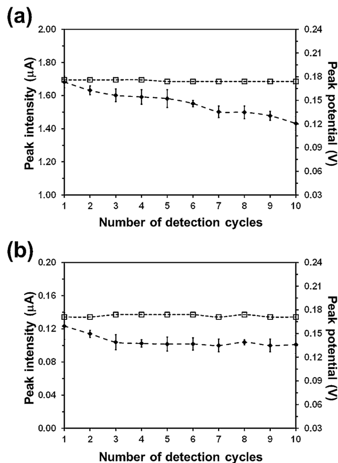
Fig. 4. Variation of the peak intensity (filled diamonds) and peak potential (empty squares) against the number of consecutive detection cycles of 100 \mu\text{M} DA using plasma treated (a) PEDOT- and (b) LDPE-modified electrodes. All experiments were performed in quadruplicate using independent electrodes. Error bars correspond to the standard deviations of independent measures.
