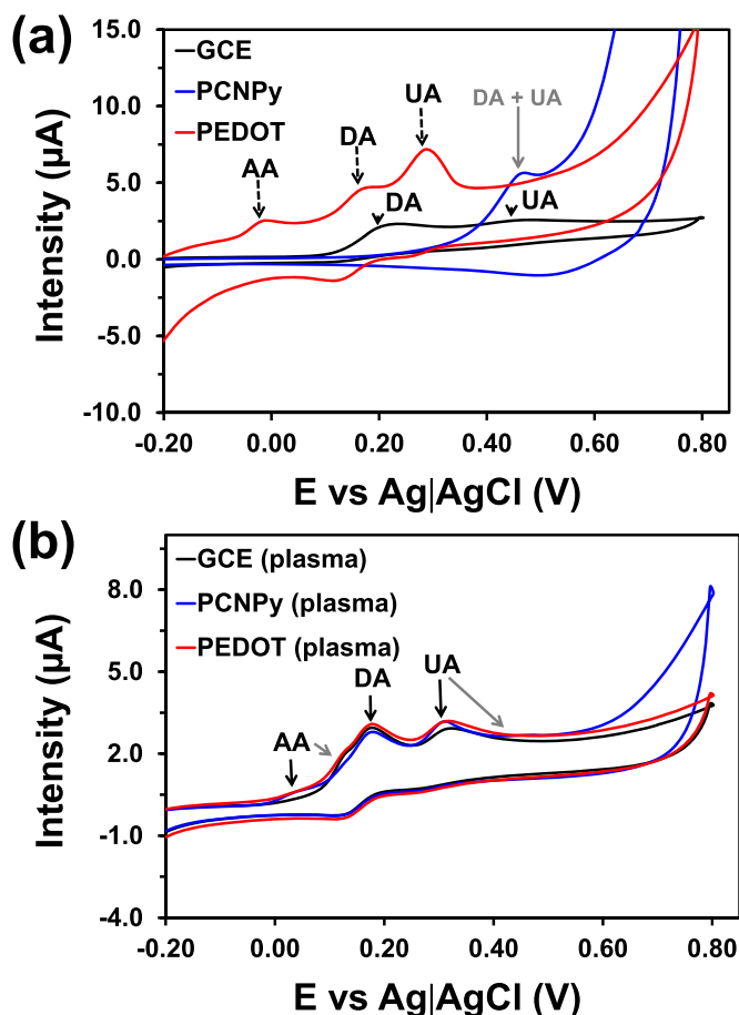
Fig. 1. Control voltammograms of DA, UA and AA ( 100\ \mu\text{M} each) in 0.1\ \text{M} PBS at (a) untreated and (b) air-plasma treated bare GCE, and both PCNPY- and PEDOT-modified GCE. Grey arrows in (b) indicate secondary oxidation processes (see text). Scan rate: 100\ \text{mV/s} . (For interpretation of the references to colour in this figure legend, the reader is referred to the web version of this article.)
