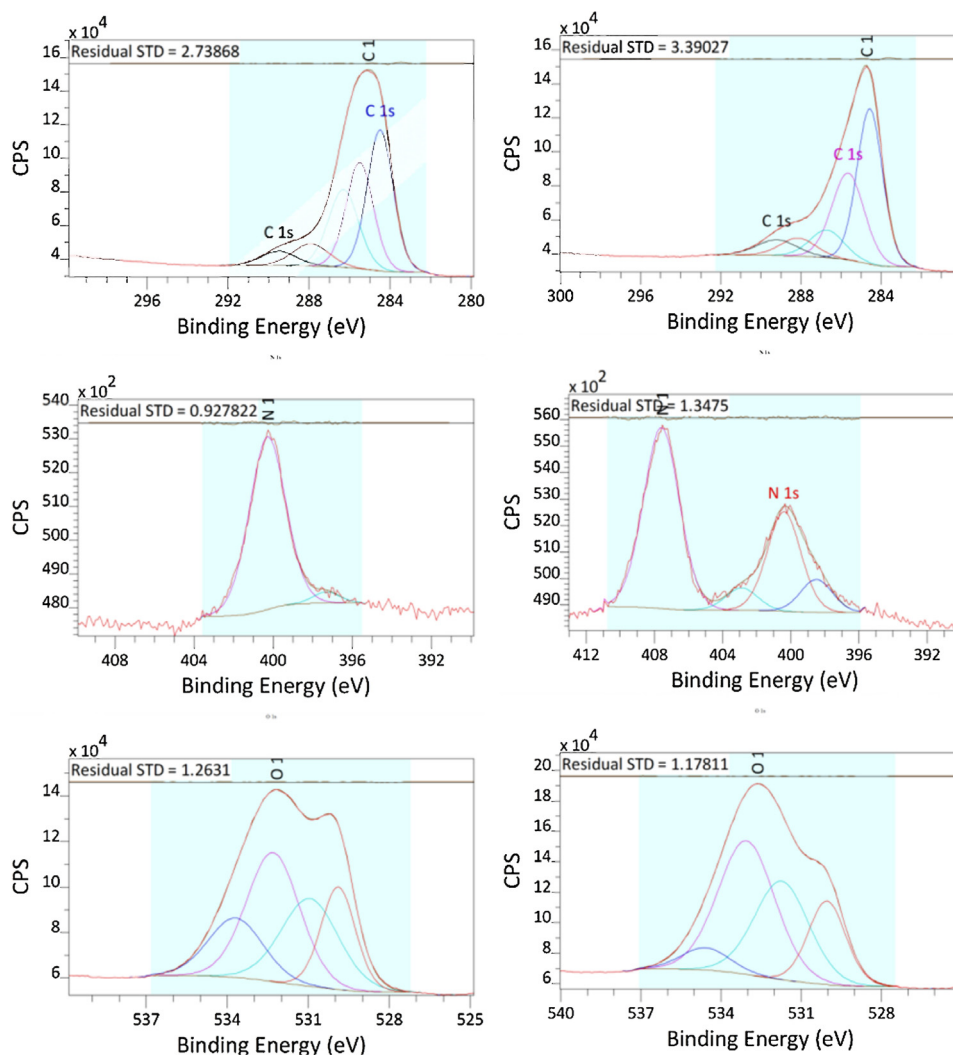
Fig. 6. C 1s, O 1s and N 1s XPS spectra of bare glassy carbon as prepared (left) and after 1 min plasma (right).
