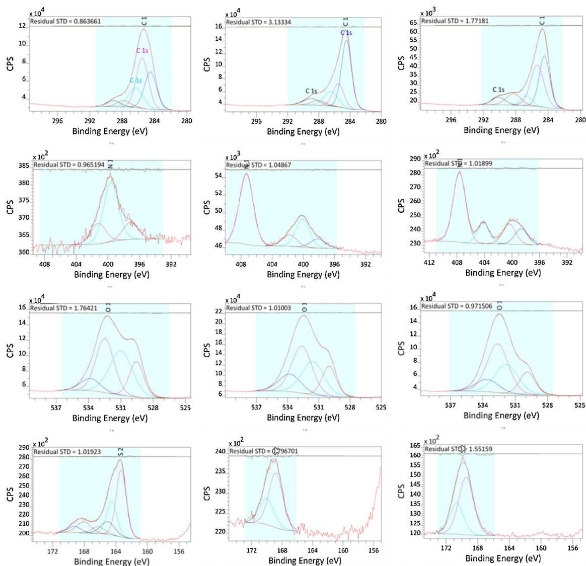
Fig. 7. C 1s, O 1s, N 1s and S 2p XPS spectra of PEDOT untreated (left) and after plasma-treatment using t_{cp} = 1 min (center) and t_{cp} = 2 min (right).
