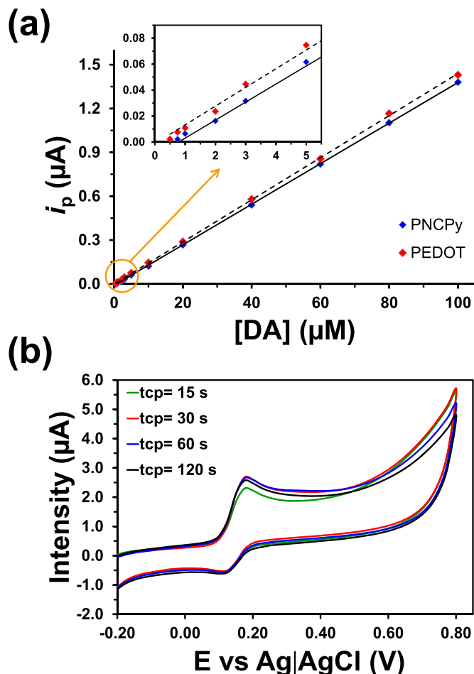
Fig. 2. (a) DA detection limit of PEDOT- and PCNPY-modified GCEs with cold-plasma treatment, as obtained from the standard addition of 10\ \mu\text{L} of DA to 10\ \text{mL} of 0.1\ \text{M} PBS. The anodic peak intensity ( i_p ) was determined by CV using a scan rate of 50\ \text{mV s}^{-1} . (b) Control voltammograms of 100\ \mu\text{M} DA in 0.1\ \text{M} PBS at cold-plasma treated PEDOT-modified GCE prepared using different t_{cp} values. Scan rate: 100\ \text{mV/s} .
