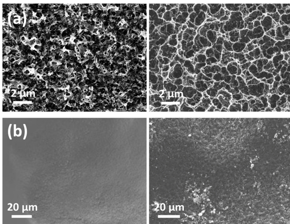
Fig. 8. SEM micrographs of (a) PEDOT and (b) PNCpY before (left) and after (right) plasma treatment using t_{cp} = 2 min.
