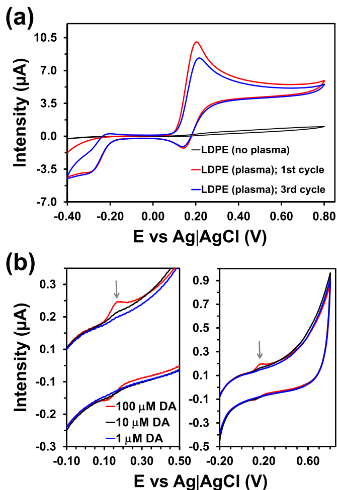
Fig. 3. (a) Control voltammogram of 1 mM DA in 0.1 M PBS at LDPE-modified GCE. Voltammograms recorded using untreated electrodes (black) and cold-plasma treated electrodes (red: first detection cycle; blue: third detection cycle). (b) Control voltammograms of 100, 10 and 1 \mu\text{M} DA at cold-plasma treated LDPE-modified GCEs. Right: complete voltammograms; Left: magnification of the region associated to the oxidation of DA molecules. In all cases: scan rate: 100 mV/s. Initial and final potentials: -0.40 V; reversal potential: +0.80 V. (For interpretation of the references to colour in this figure legend, the reader is referred to the web version of this article.)
