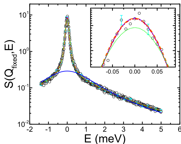
Figure 3. (Color online) Fits to the synthetic QENS data (black circles) using an increasing number of L modes: L1 (solid blue line), L2 (dotted green), L3 (dashed-dot red), L4 (dashed orange), and L5 (solid purple). Note the logarithmic (linear) scales on the main figure (inset).
